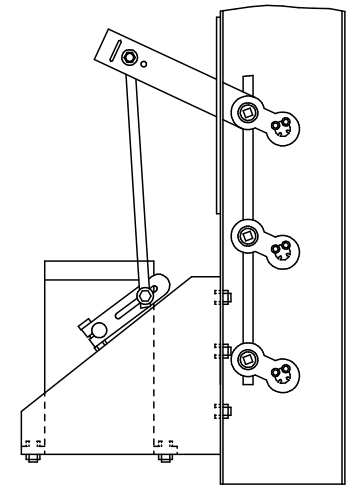
TYPICAL LOUVER DRIVE
