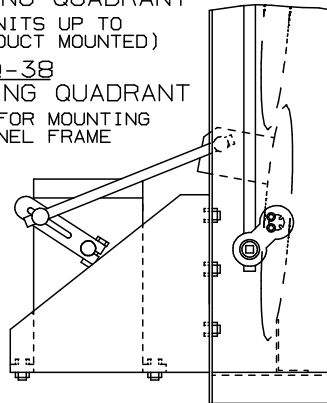
TYPICAL DAMPER DRIVE
